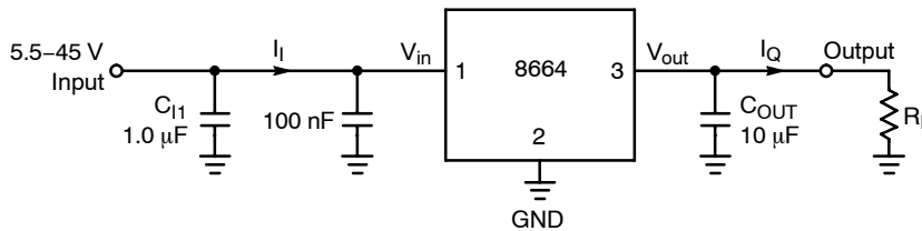
Figure 2. Measurement Circuit
