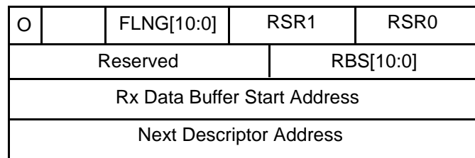
Figure 3.3 The Receive Descriptor Format
