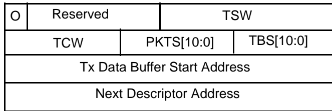
Figure 3.2 The Transmit Descriptor Format
