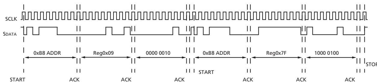
Figure 18: Timing Diagram Showing a Bytewise Write to Reg0x09 with Value 0x0284
