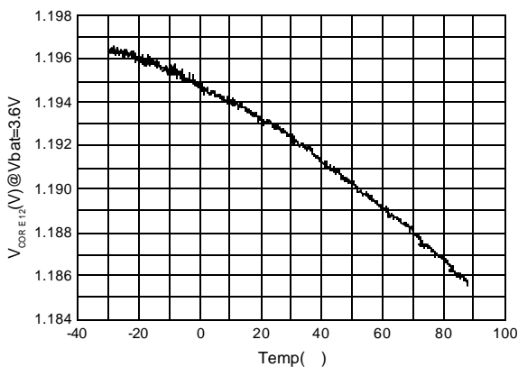
V CORE12 vs. Temp
