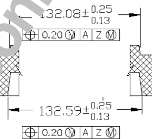
SECTION J-J
