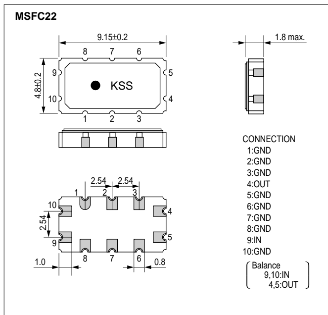
Dimensions(mm)
