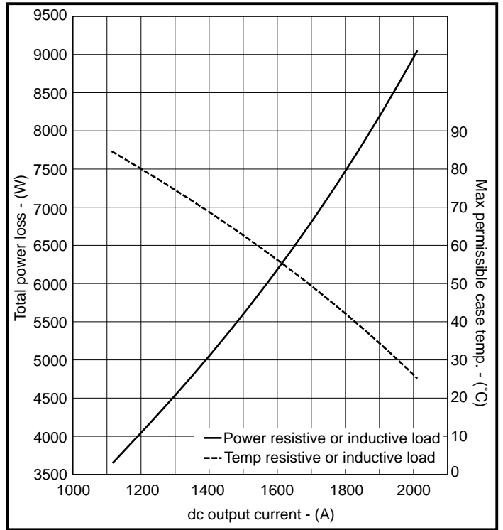
Fig. 12 50/60Hz three phase bridge DC output current vs power loss and maximum permissible case temperature
