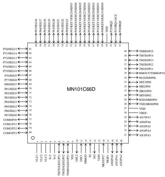
LQFP080-P-1414A *Lead-free TQFP080-P-1212D *Lead-free (under planning)
