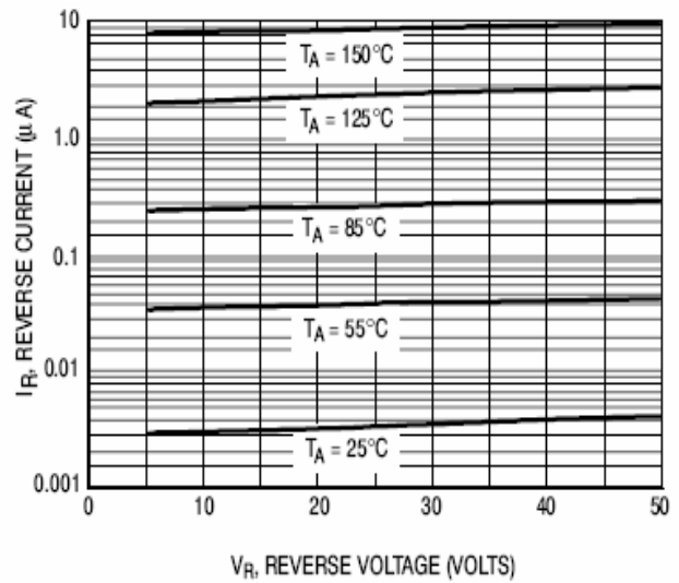
Figure 2. Leakage Current
