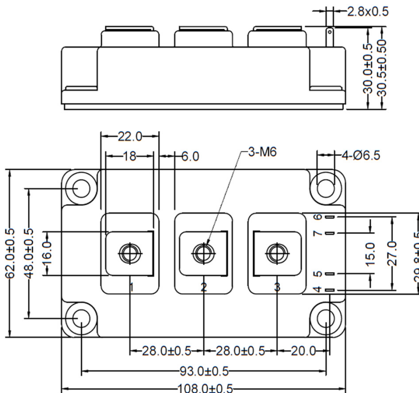
Figure 14. Package Outline
