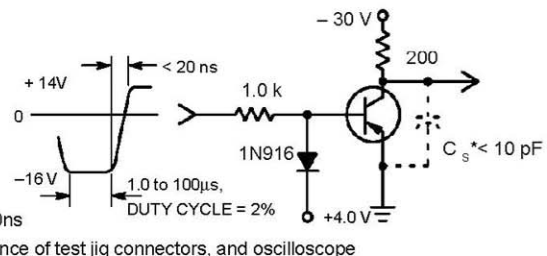
Figure 2. Turn–Off Time
