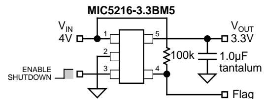
3.3V Low-Noise Regulator
