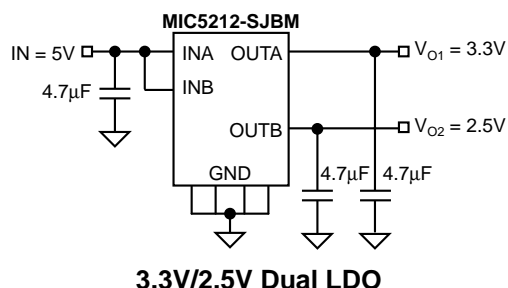
3.3V/2.5V Dual LDO
