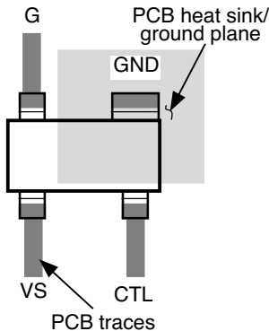
Figure 4. Heat-Sink Plane
