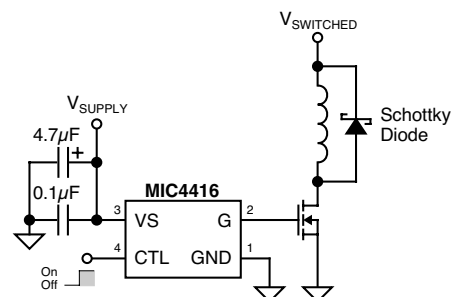
Figure 3. Switching an Inductive Load
