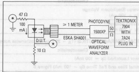
Figure 5. Optical Rise and Fall Time Test Set (10%-90%)
