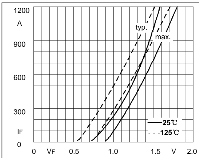
Fig5. Forward Characteristics
