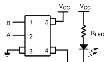
Figure 8. LED Driver
