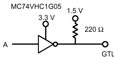
Figure 9. GTL Driver
