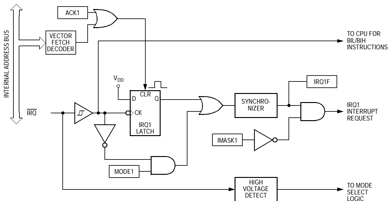
Figure 16-1. IRQ Block Diagram
