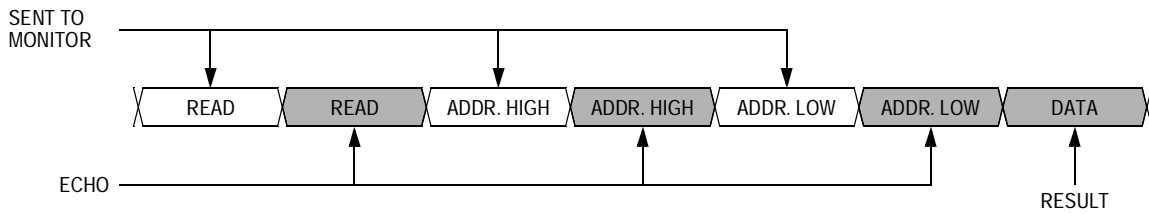
Figure 13-4. Read Transaction
