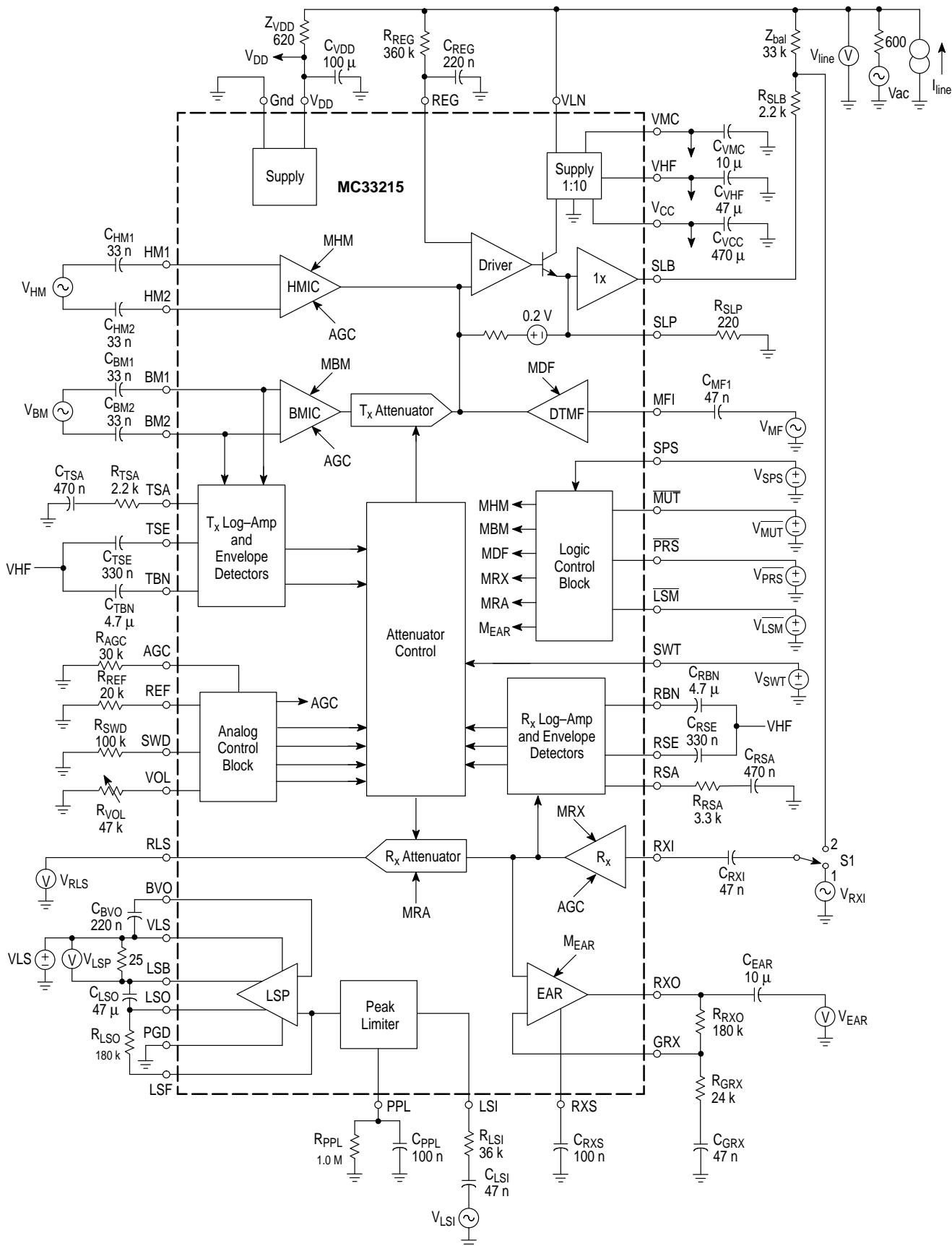
Figure 17. Test Circuit
