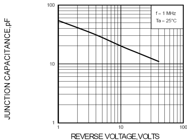
FIG.5-TYPICAL JUNCTION CAPACITANCE
