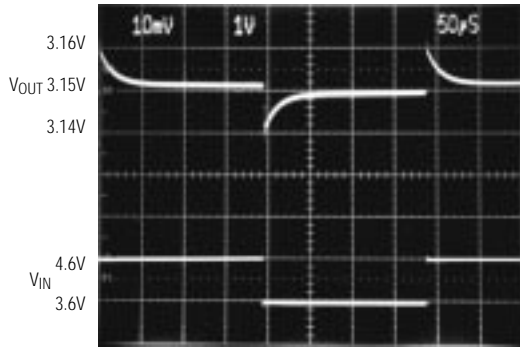
I_{LOAD} = 50mA , V_{OUT} IS AC COUPLED
