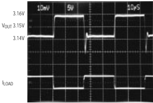
V_{IN} = V_{OUT} + 0.2V , I_{LOAD} = 0mA to 50mA , C_{IN} = 10\mu F , V_{OUT} IS AC COUPLED
