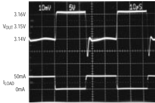
V_{IN} = V_{OUT} + 0.1V , I_{LOAD} = 0mA to 50mA , C_{IN} = 10\mu F , V_{OUT} IS AC COUPLED
