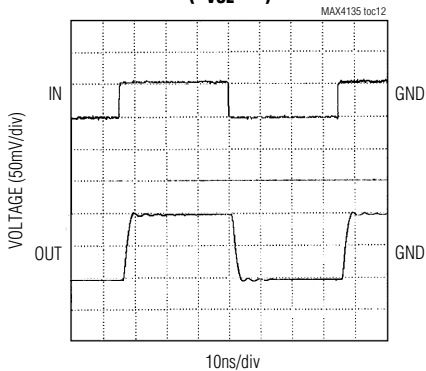
MAX4135 SMALL-SIGNAL PULSE RESPONSE ( A_{vCL} = 2 )
