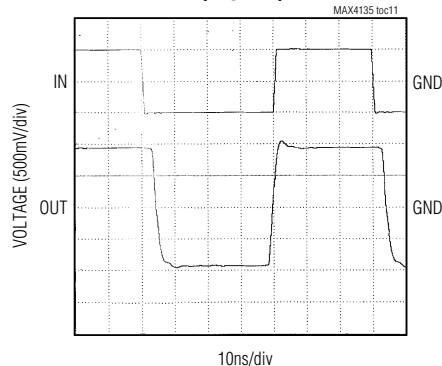
MAX4136 LARGE-SIGNAL PULSE RESPONSE ( A_{vCL} = 2 )
