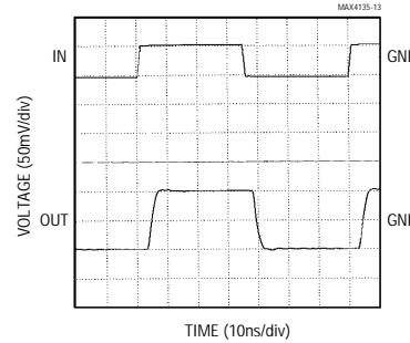
MAX4136 SMALL-SIGNAL PULSE RESPONSE ( A_{VCL} = +2 )
