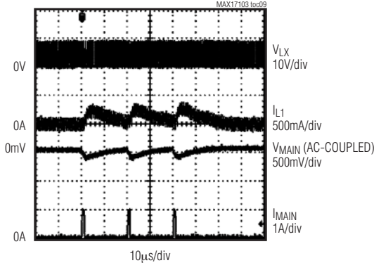
STEP-UP REGULATOR PULSED LOAD-TRANSIENT RESPONSE (20mA TO 1A)
