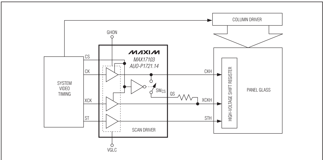
Figure 4. Scan Driver System Diagram
