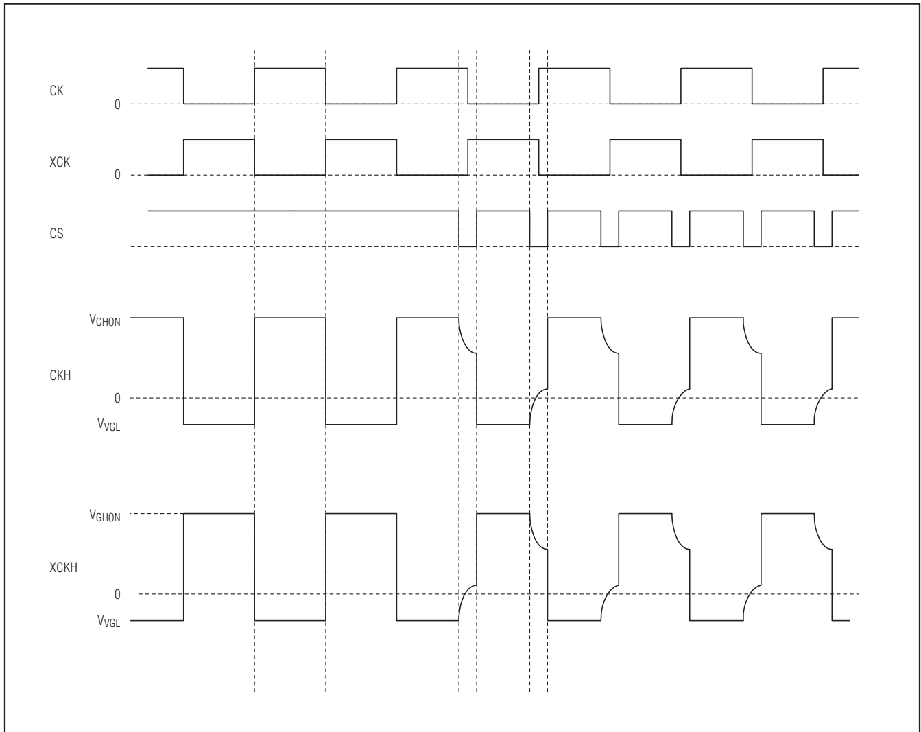
Figure 5. Scan Driver System Timing Utilizing Charge Sharing Between the CKH and XCKH Outputs
