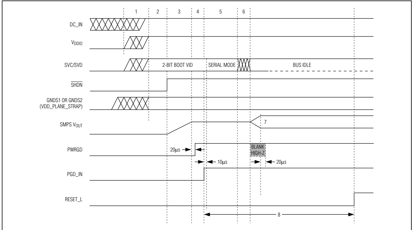
Figure 7. Startup Sequence
