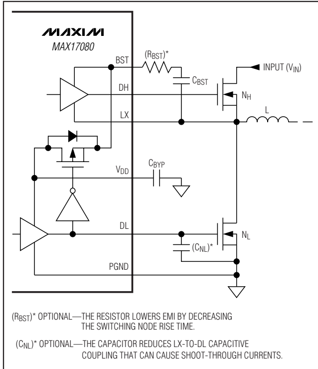
Figure 10. Gate-Drive Circuit
