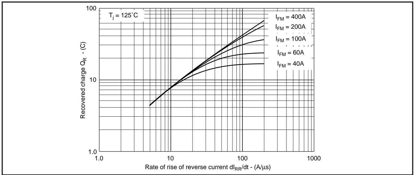
Fig.7 Recovered charge (diode only)
