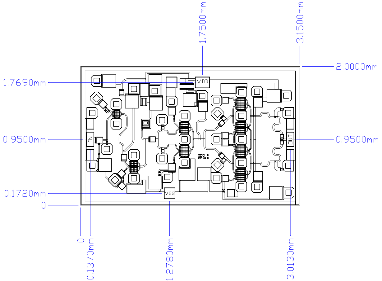
Chip edge to bond pad dimensions are shown to the center of the bond pad.
