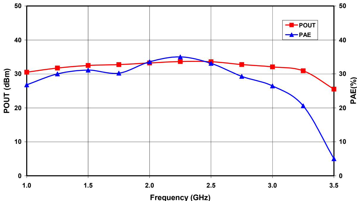
Figure 1. Output Power and Power Added Efficiency vs. Frequency at V_{DD} = 8V and P_{in} = 18 dBm.
