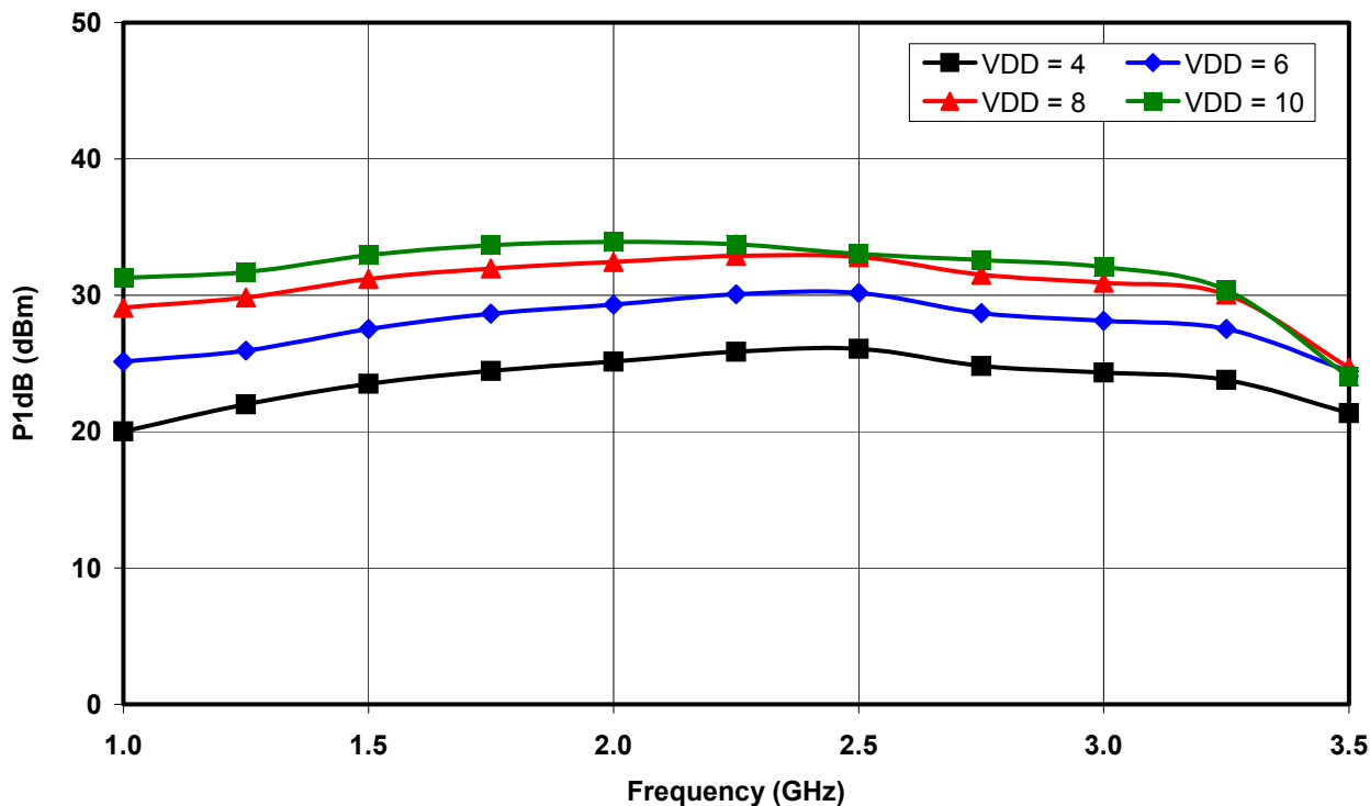
Figure 3. 1dB Compression Point vs. Frequency
