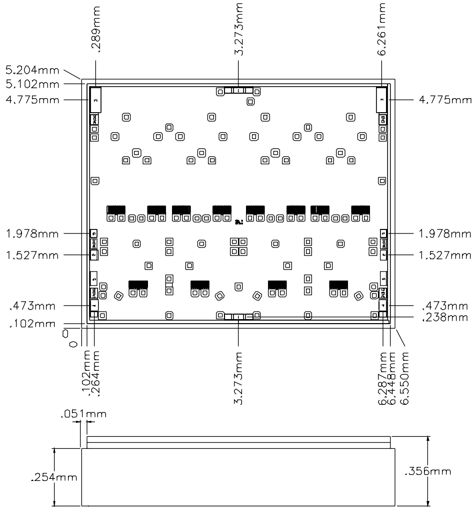
Figure 17. Die Layout
