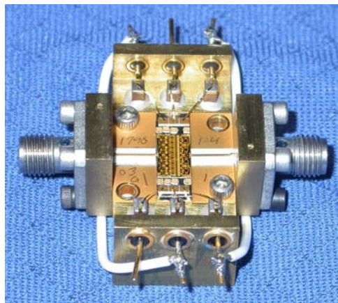
Figure 16. Fixture used to characterize MAAPGM078-DIE under CW stimulus.
