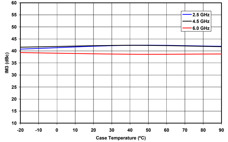
Figure 26. Third Order Intermod vs. Case Temperature and Frequency at Single Carrier Output Power Level = 16 dBm, VD = 8V and IDQ = 660mA
