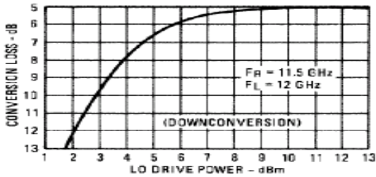
Conversion Loss vs. LO Drive
