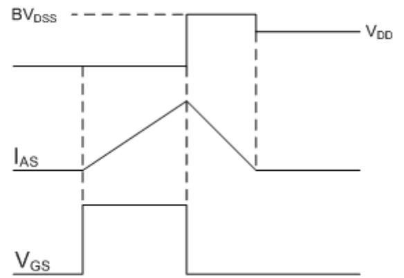
Fig.12 Unclamped Inductive Switching Test Circuit & Waveforms
