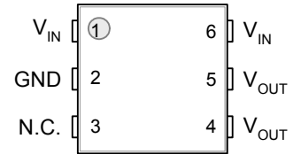
LM PACKAGE (Top View)
