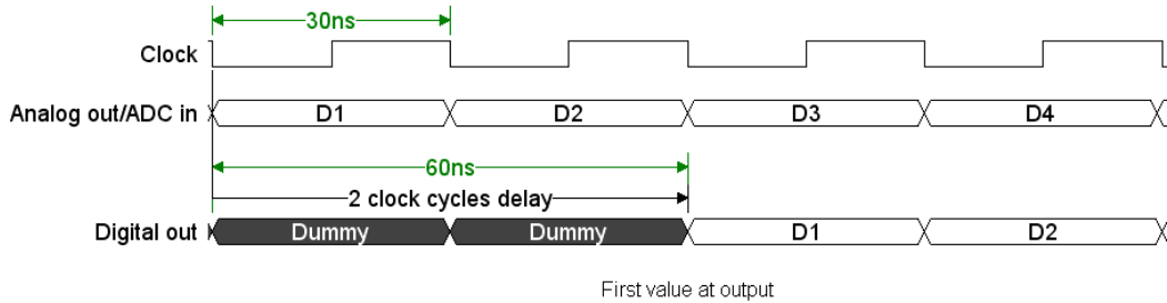
Figure 6: ADC timing
