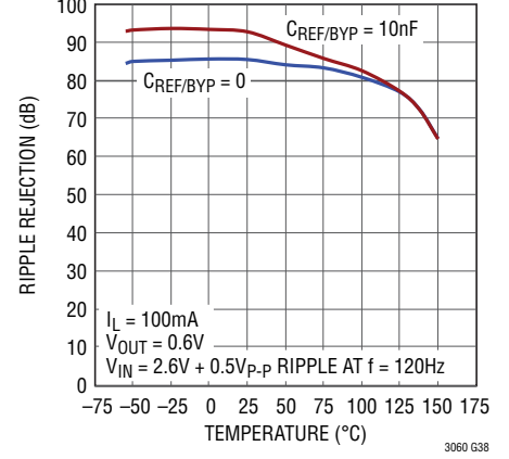
Ripple Rejection vs Temperature
