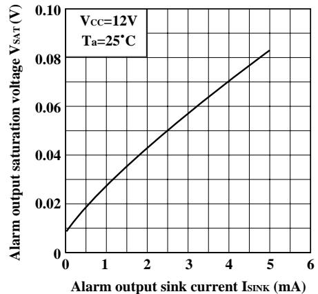
Fig. 8 Alarm Output Saturation Voltage vs. Alarm Output Sink Current
