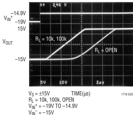
Below V_S^- Fault (Rising)
