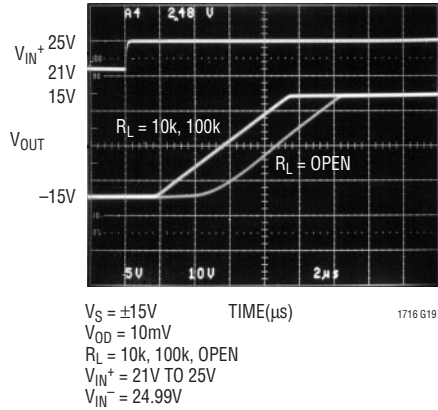
Response Time
