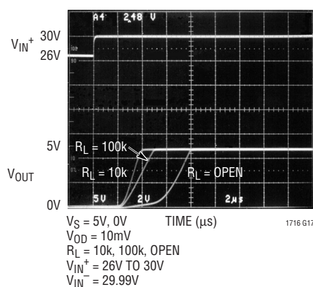
Response Time
