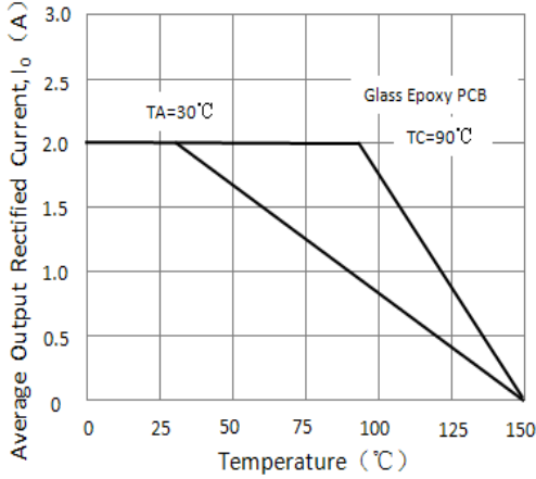
Figure 1. Output Rectifier Current Derating Curve
