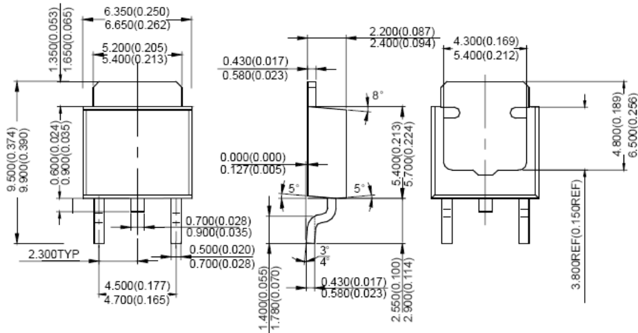
D-PACK (TO-252)
