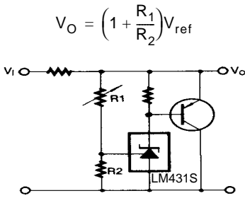
Figure 15. High Current Shunt Regulator
