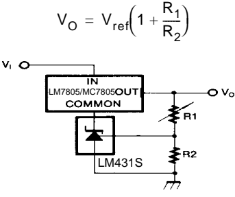
Figure 14. Output Control for Three-Termianl Fixed Regulator
