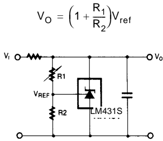
Figure 13. Shunt Regulator
