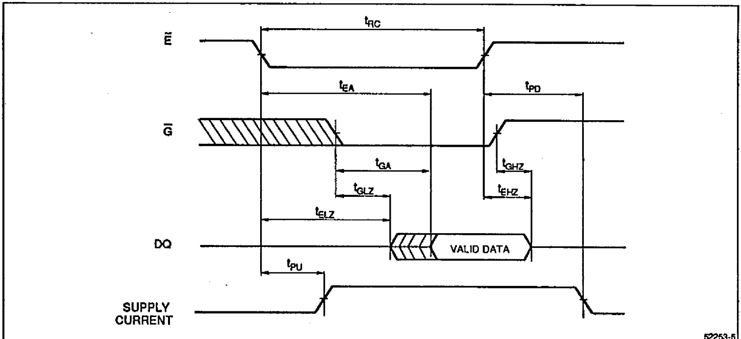
Figure 5. Read Cycle No. 2
