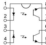
LDA201 Pinout
