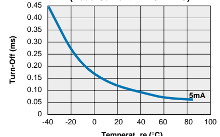
LCA127 Typical Turn-Off vs. Temperature (Load Current = 170mADC)
