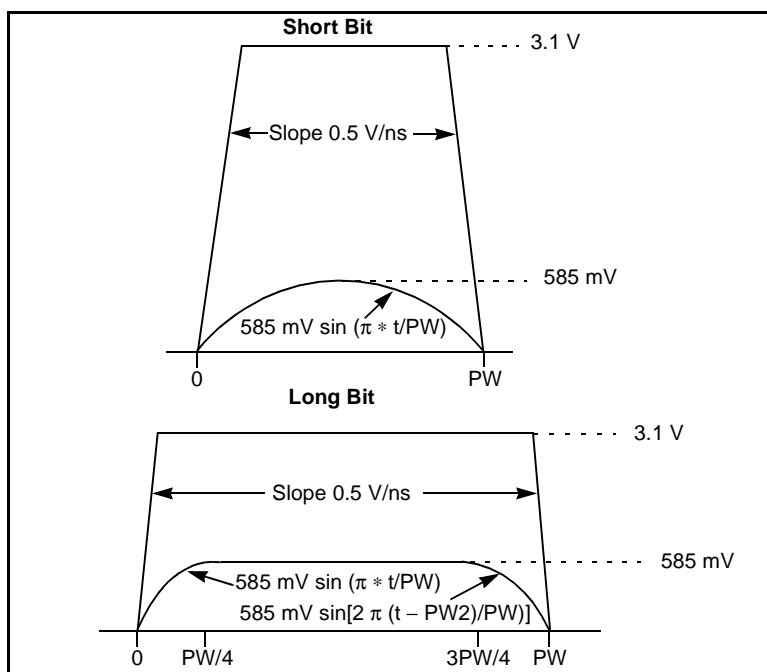
Figure 1.5 TP Input Voltage Template (10 Mb/s)
