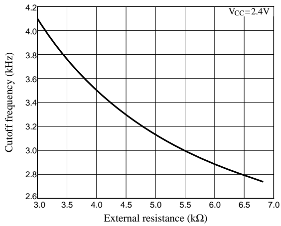
Graph 1. Splatter Filter Cutoff Frequency vs. External Resistance
