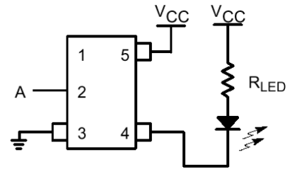
Figure 8. LED Driver
