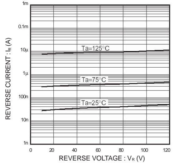
Fig.2 Reverse characteristics
