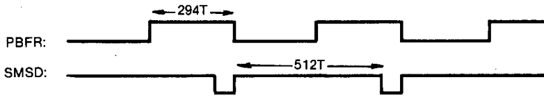
(b) Timing chart of SMSD output when PBFR is "294T"
