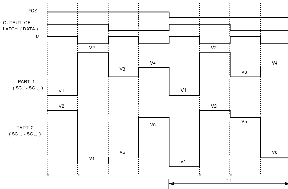
Fig. 6. Output waveform
