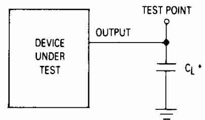
Figure 2. Test Circuit
